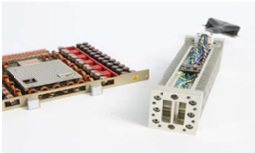
Phase shifter
