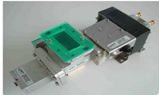
Fast Ferrite Tuners / I-Q-modulators
